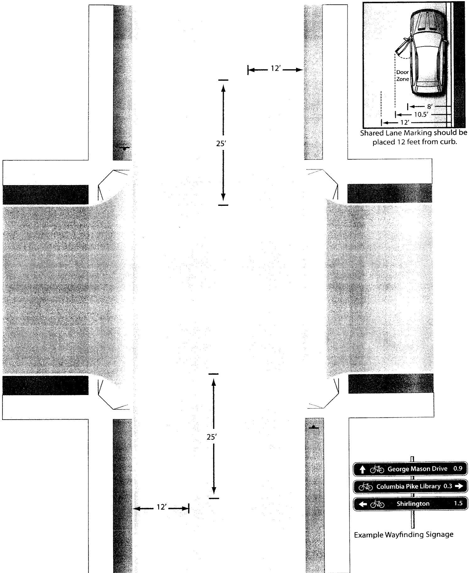
Standard Bike Boulevard Intersection 9th and 12th Streets
